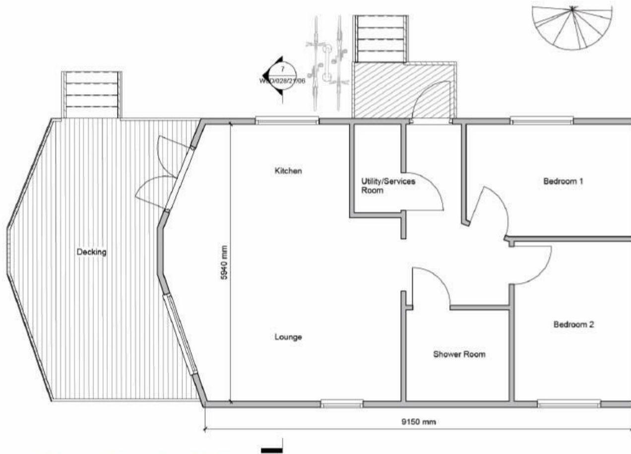
Proposed Floorplans of Cabin
