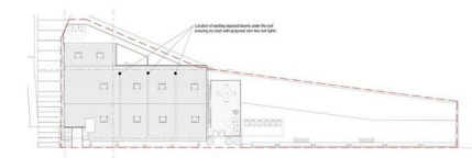
2 Proposed First Floor (Kings Road Level)
