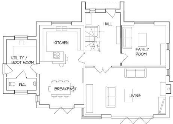
PLOT 3 GROUND FLOOR 106 sq.m / 1141 sq.ft.
