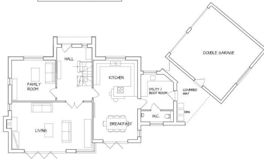
PLOT 2 GROUND FLOOR 106 sq.m / 1141 sq.ft.
