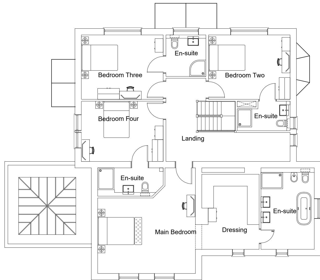
First Floor Plan (143m 2 - 1539sqft)
