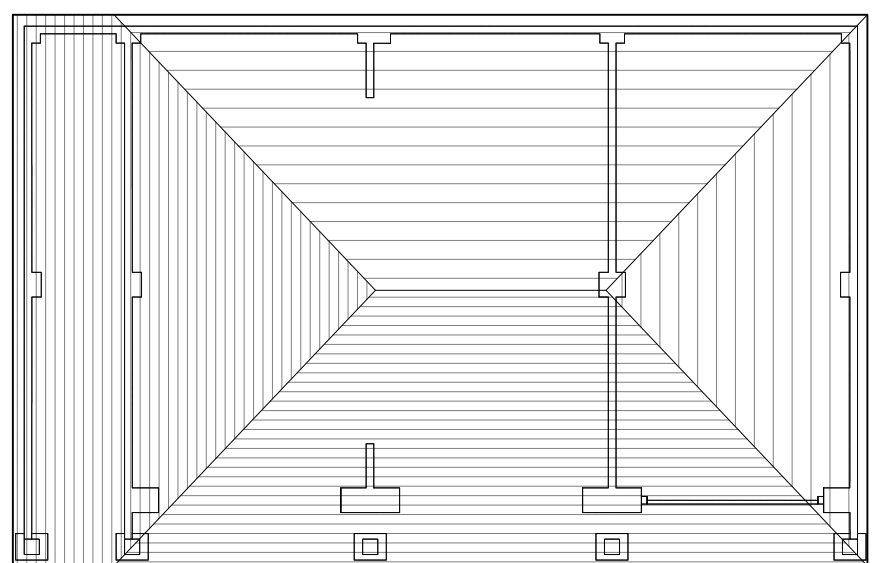
Roof Plan
